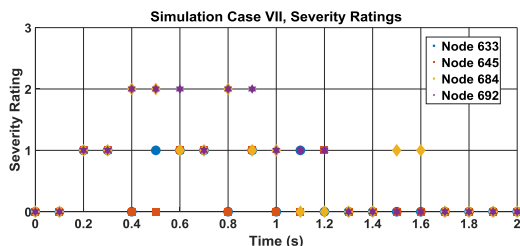
Fig. 23. Node severity ratings for Simulation Case VII
