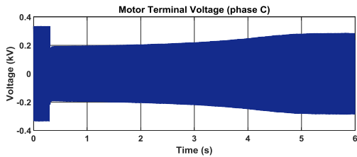
Fig. 19. Voltage at Node 634(phase C) during motor starting event.
