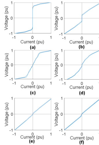
Fig. 6. Different HIF V-I Characteristics obtained from the same HIF model resembling real-field data: (a) Concrete, (b) Wet grass, (c) Dry tiles, (d) Damp sand, (e) Dry rubber and (f) Damp tiles
