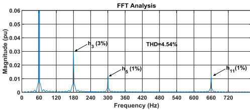
Fig. 13. FFT of grid voltage with injected harmonics (Simulation Case I, Scenario C)
