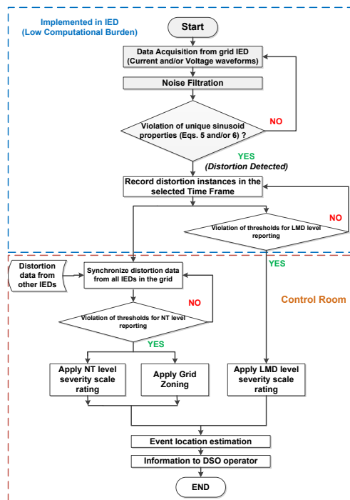
Fig. 3. ADDT Implementation Flowchart
