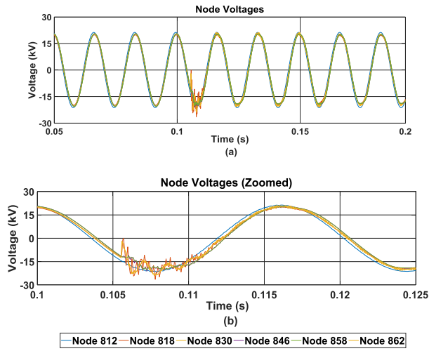
Fig. 9. Measured voltages at different measurement points for Simulation Case II, Scenario B. HIF event and capacitor and load switching occur at t=0.105s . (a) Node Voltages, (b) Node Voltages (Zoomed)
